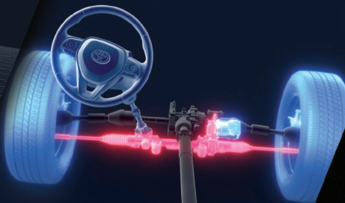
Parallel Rack Power Steering with Speed Sensitive Function
